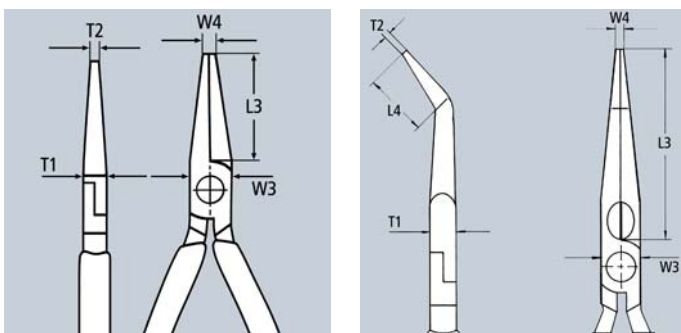
26 27 200 ⚡ 1000 V ⚠️ ⚙️ ⚡ ⚙️ ⚡ ⚙️ ∠40°
