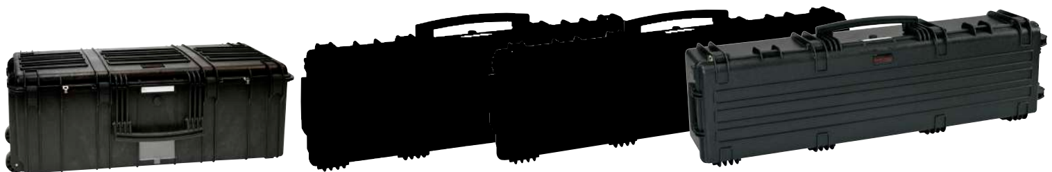
9433 Int. Dim. 936x350x330 mm. 36 7/8 x 13 3/4 x 13 in 11413 Int. Dim. 1136x350x135 mm. 44 3/4 x 13 3/4 x 5 5/16 in 13513 Int. Dim. 1350x350x135 mm. 53 1/8 x 13 3/4 x 5 5/16 in 13527 Int. Dim. 1350x350x272 mm. 53 1/8 x 13 3/4 x 10 11/16 in
