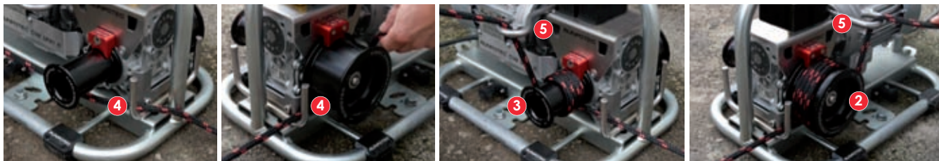
The cable to be pulled is connected, preferably with a connection swirl with swivel , with the pull rope.
