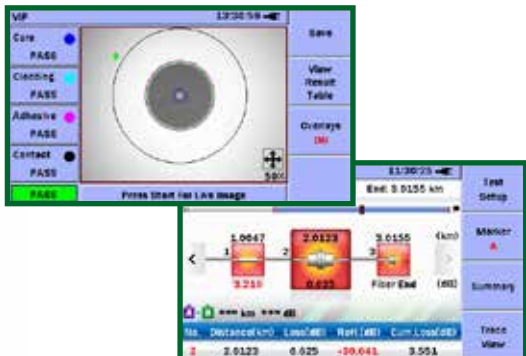
MT9090A OTDR with Fiber Visualizer Summary
