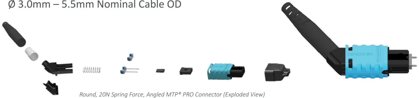
Round, 20N Spring Force, Angled MTP® PRO Connector (Exploded View)
