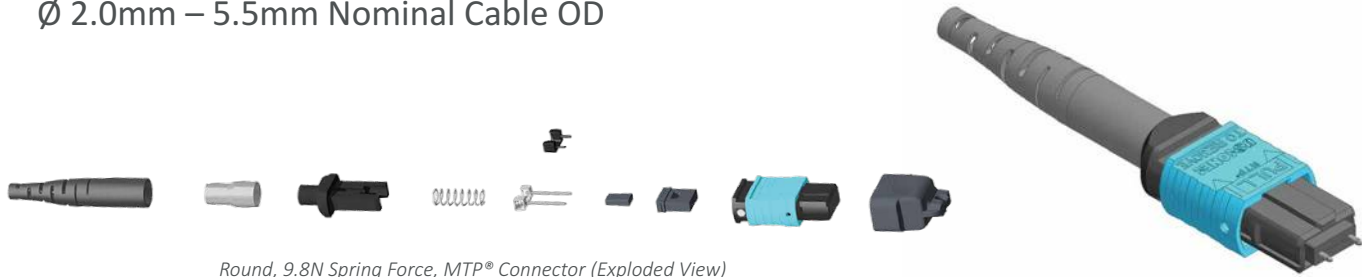
Round, 9.8N Spring Force, MTP® Connector (Exploded View)
