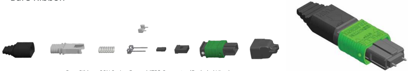
Bare Ribbon, 20N Spring Force, MTP® Connector (Exploded View)
