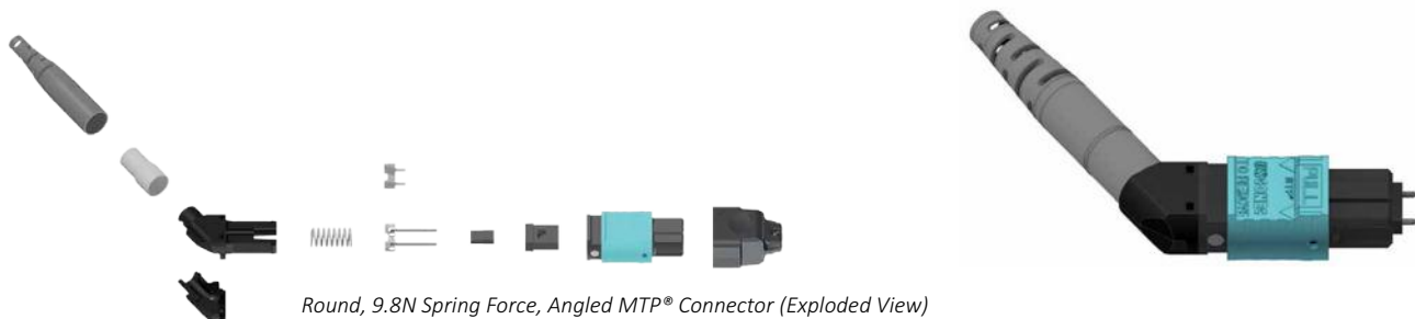
Round, 9.8N Spring Force, Angled MTP® Connector (Exploded View)
