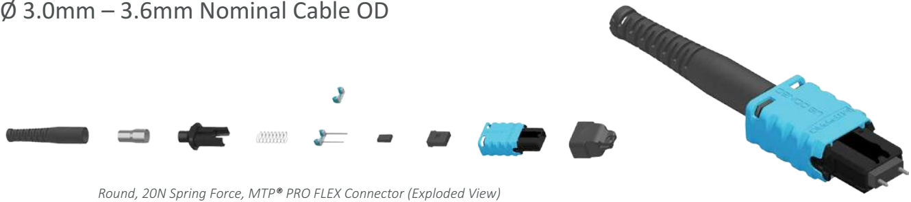
Round, 20N Spring Force, MTP® PRO FLEX Connector (Exploded View)
