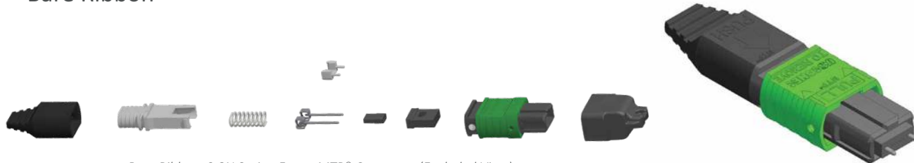
Bare Ribbon, 9.8N Spring Force, MTP® Connector (Exploded View)
