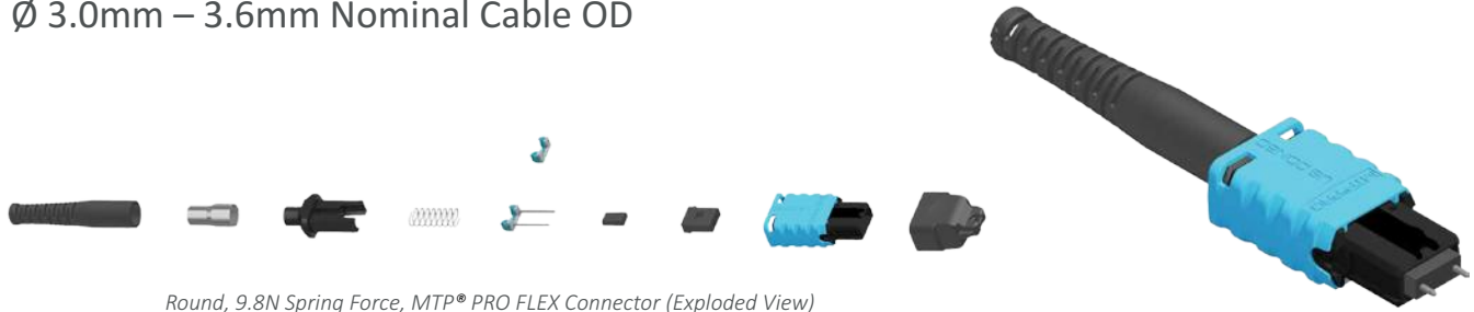
Round, 9.8N Spring Force, MTP® PRO FLEX Connector (Exploded View)
