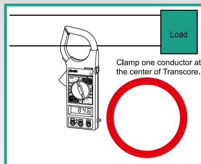
Fig.2 Correct measurement
