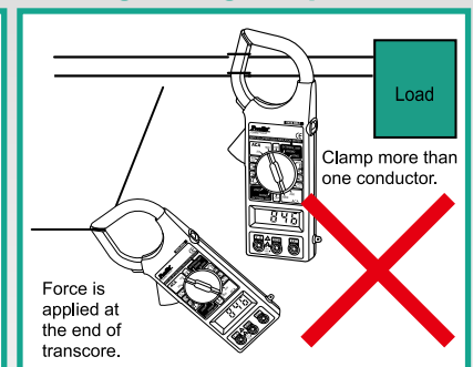
Fig.3 Wrong measurement
