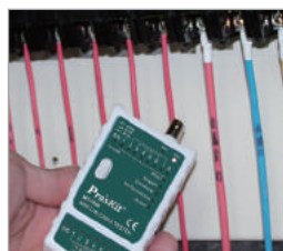
NCV detection
