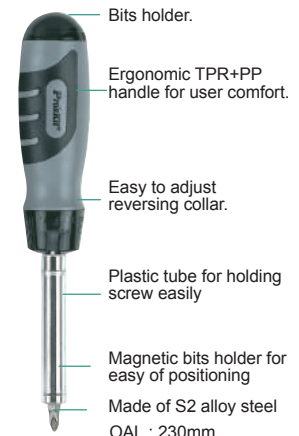
Bits holder.
